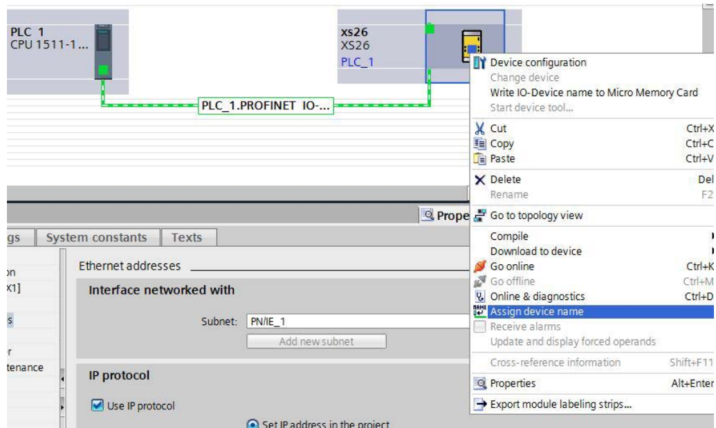
Illustration 243. Adresses Ethernet
