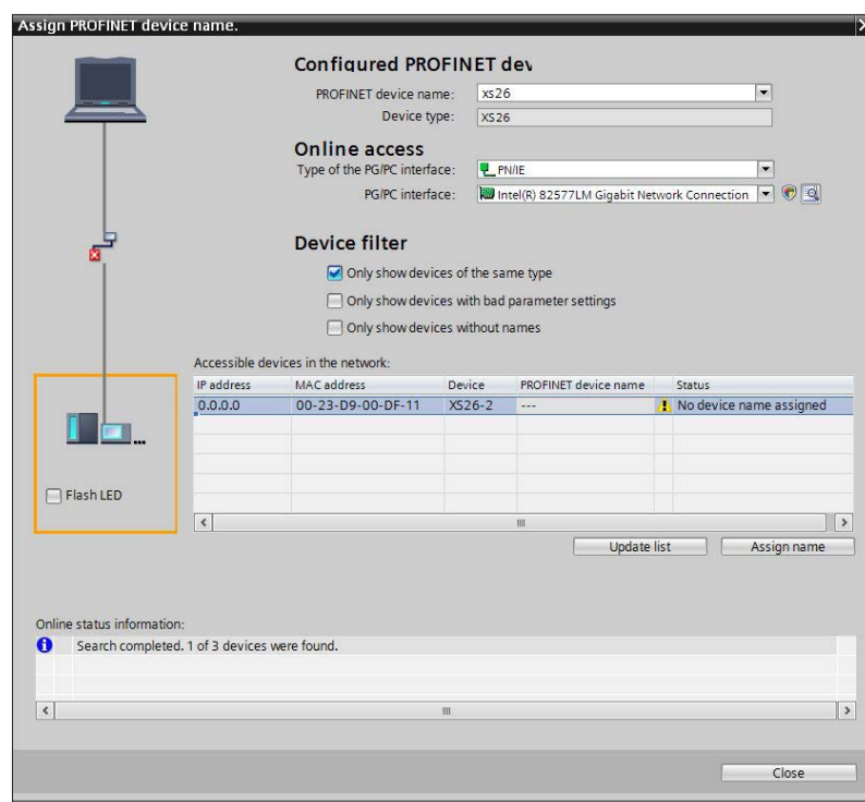
Illustration 244. Adresses Ethernet
