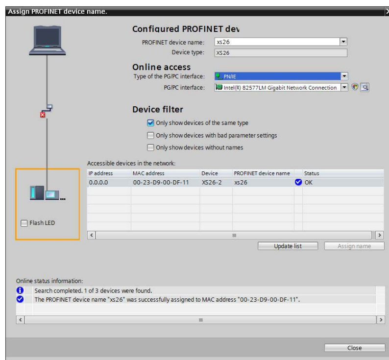
Illustration 245. Adresses Ethernet
