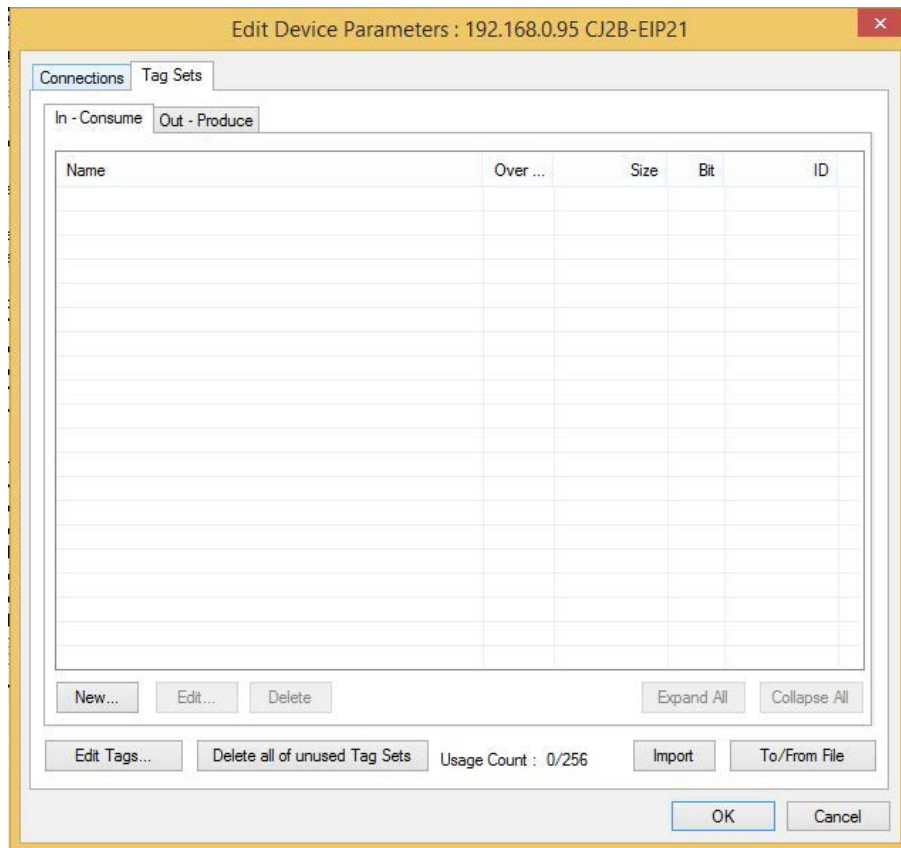
Illustration 204. Onglet Tag Sets
