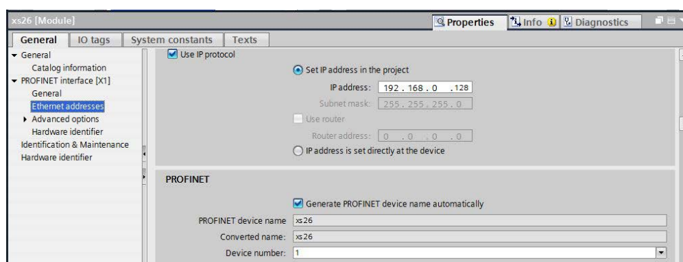
Illustration 235. Adresses Ethernet
