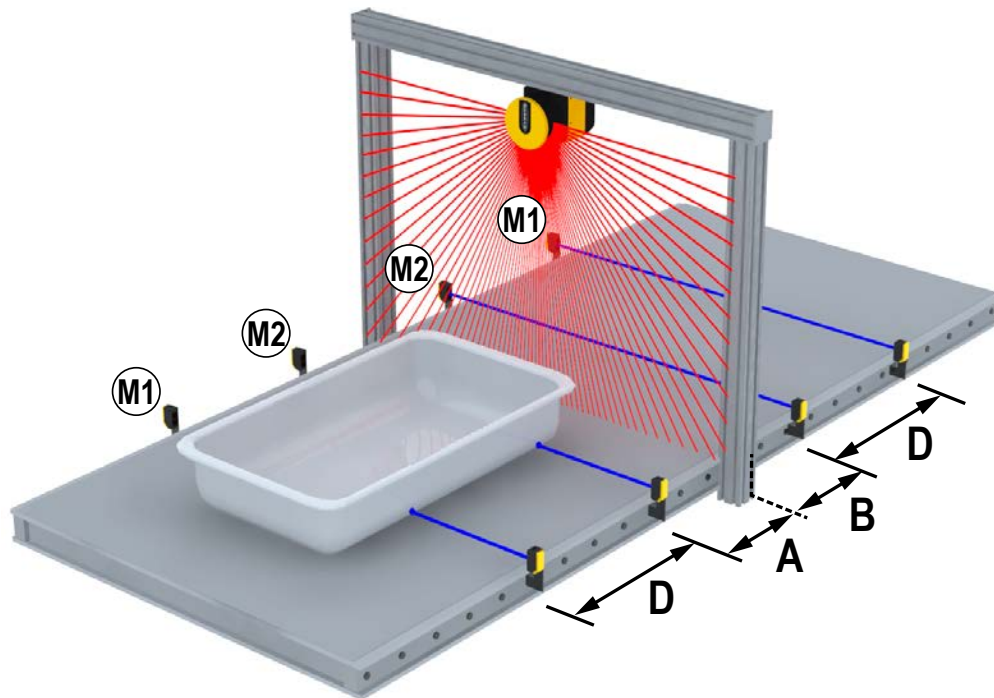
Figure 43. Muting function in the T configuration
