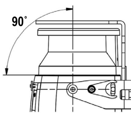
Figure 34. Adjust the scanner angle
