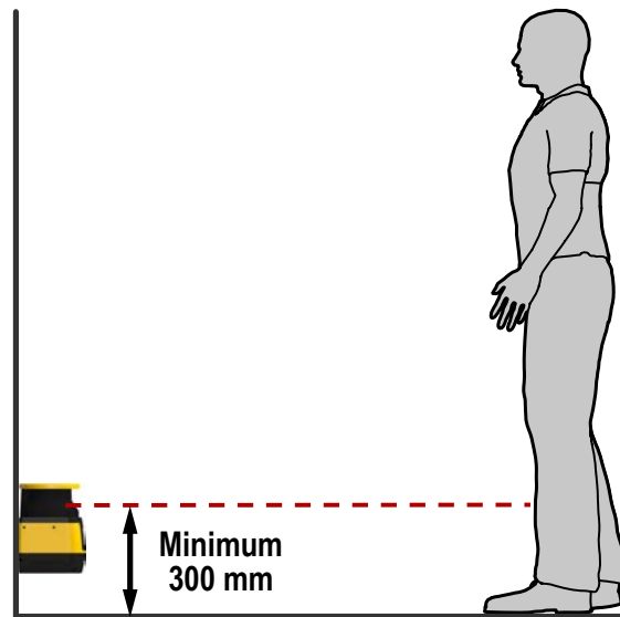
Figure 25. A zone with 70 mm resolution is mounted no lower than 300 mm above the floor
