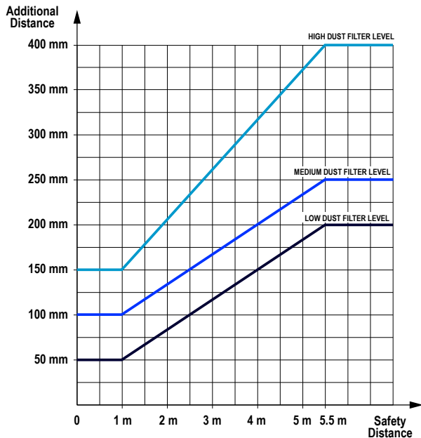
Figure 21. Additional distance for 70 mm resolution
