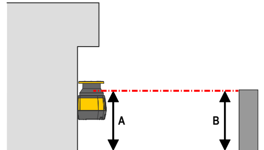
Figure 41. Safety Zone height
