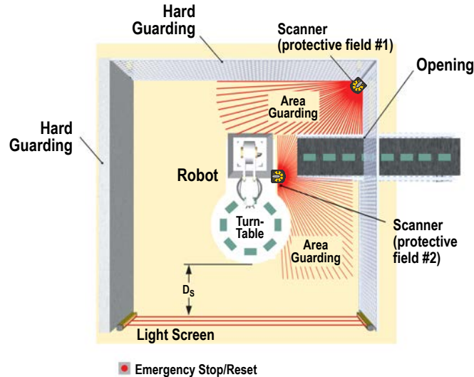
Figure 27. Supplemental safeguarding inside a robotic work cell
