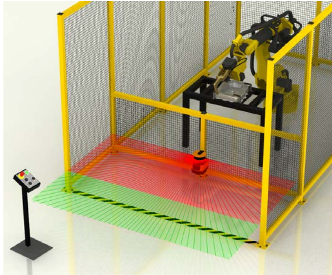
Figure 4. Horizontal stationary area guarding
