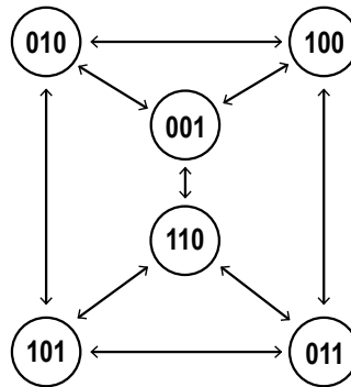
Figure 49. Switching state map
