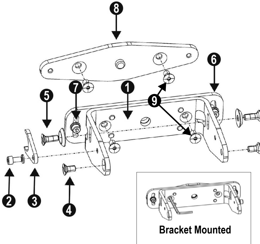
Figure 33. Pitch and roll angle adjustment bracket (SXA-MBK-1)
