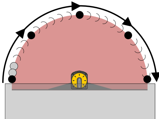
Figure 40. Safety Zone angles and locations for verification
