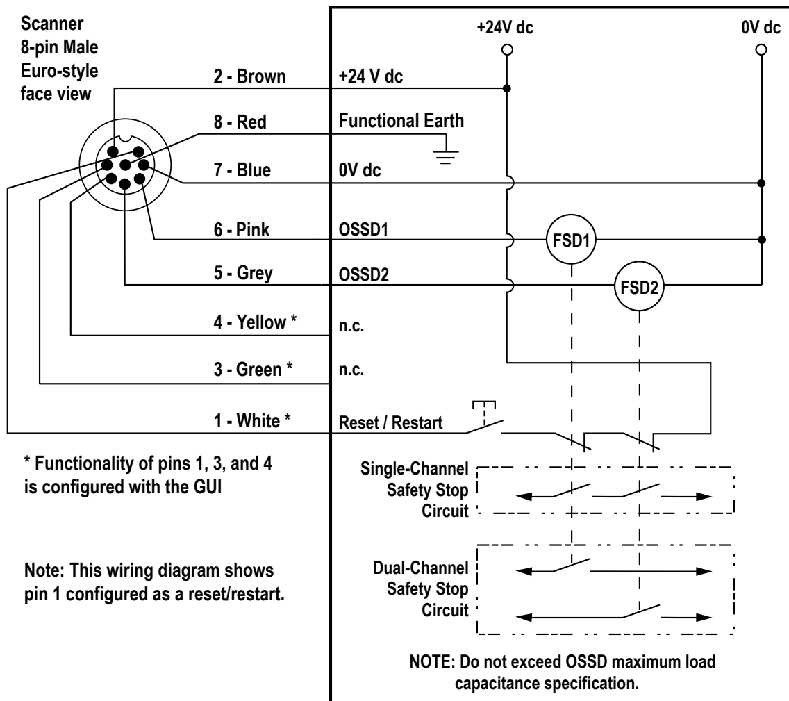
Figure 37. Wiring with FSD inputs
