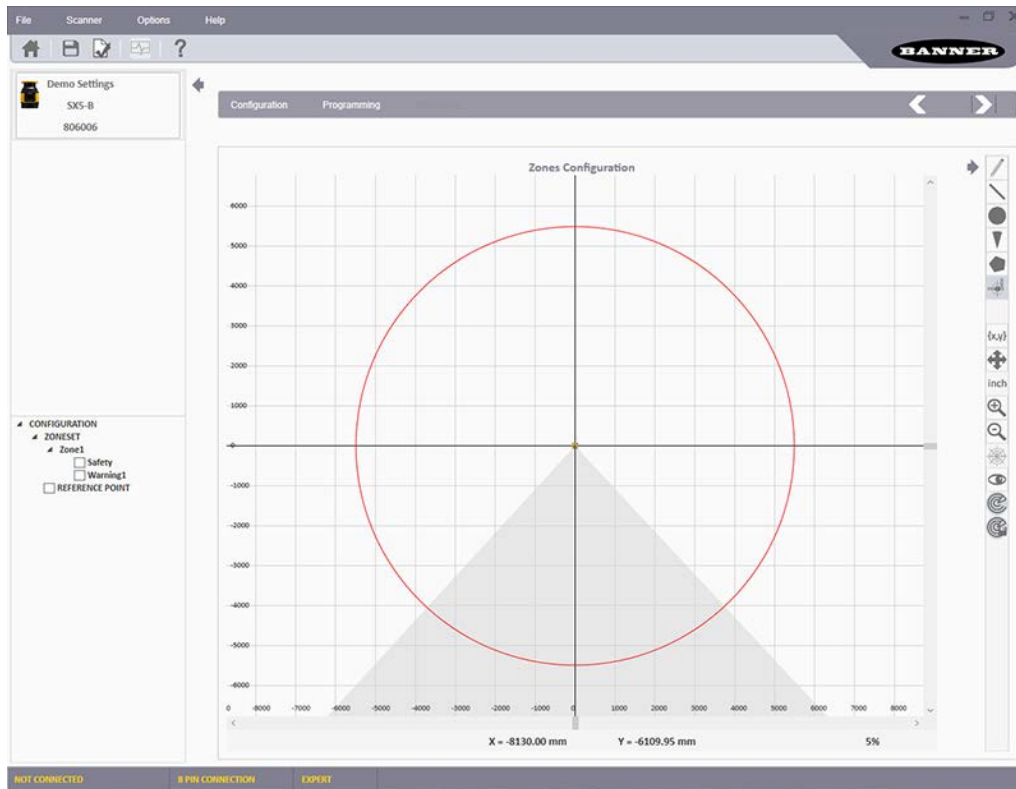
Figure 52. Zone Configuration screen
