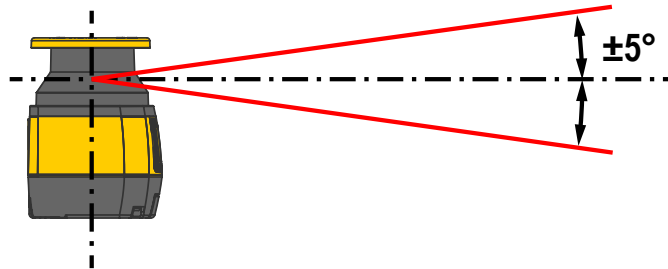
Figure 20. Position the scanner to avoid light interference
