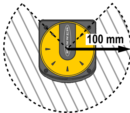
Figure 24. Limited detection capability zone
