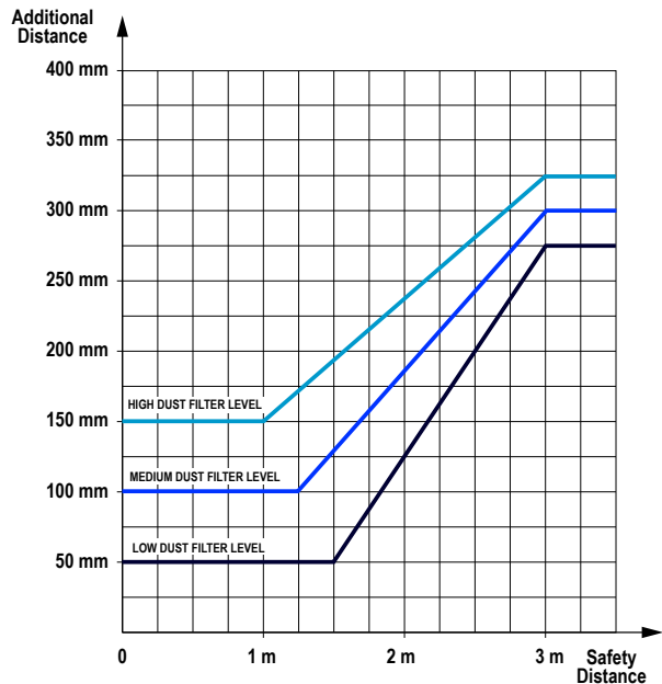
Figure 22. Additional distance for 40 mm resolution
