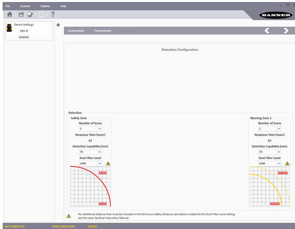
Figure 51. Detection Configuration screen
