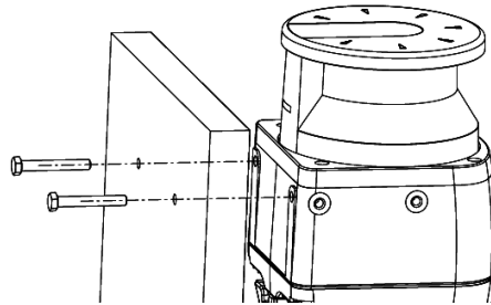
Figure 31. Mounting the scanner directly to a surface
