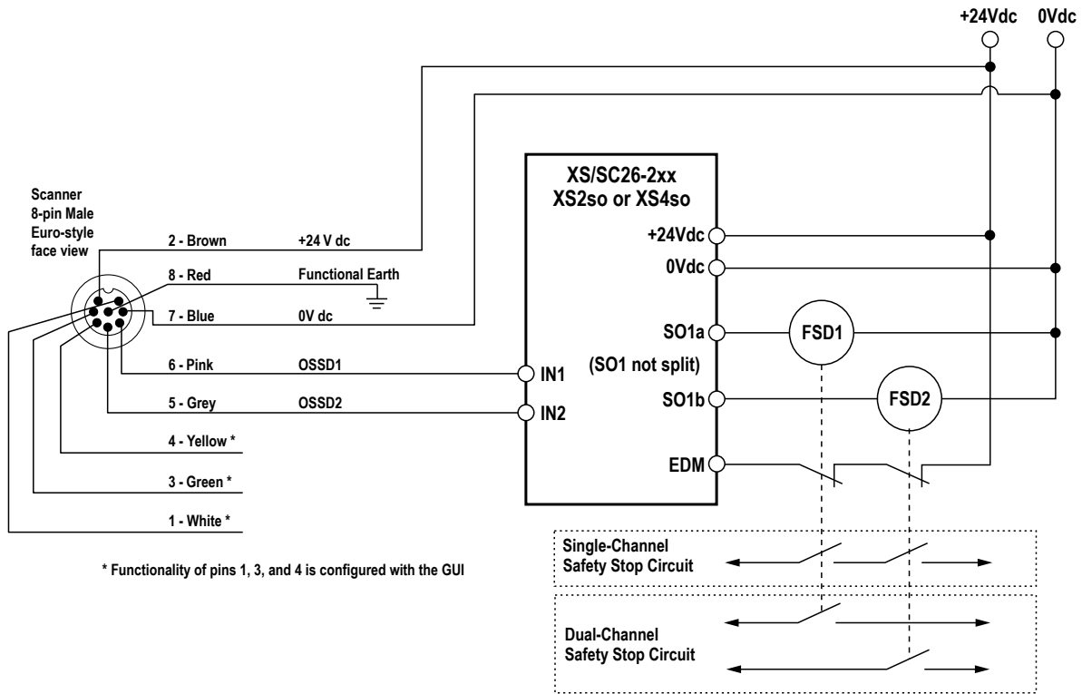
Figure 39. Wiring to a Safety Controller
