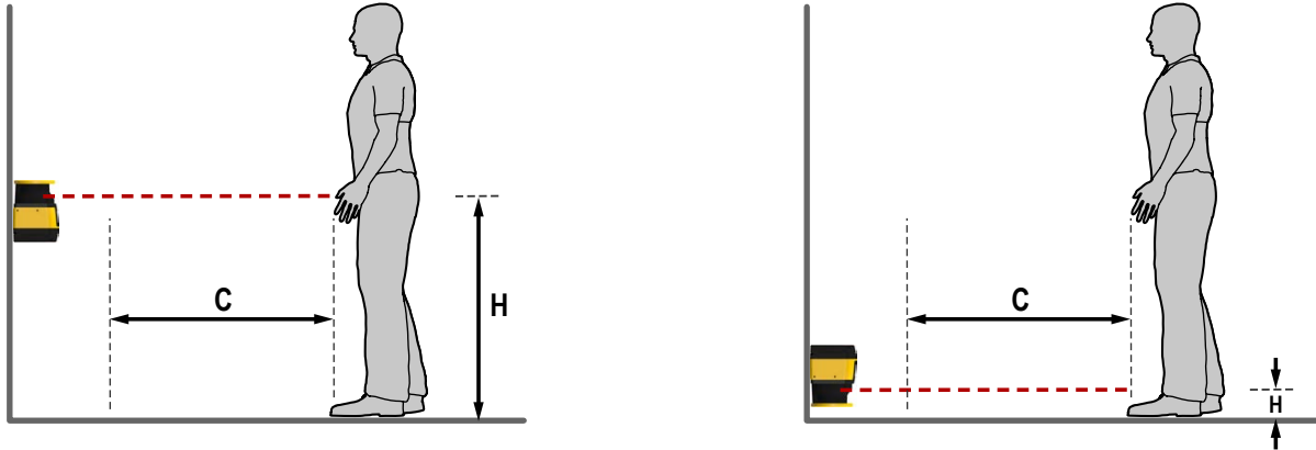
Figure 26. Calculating the safety distance for each resolution
