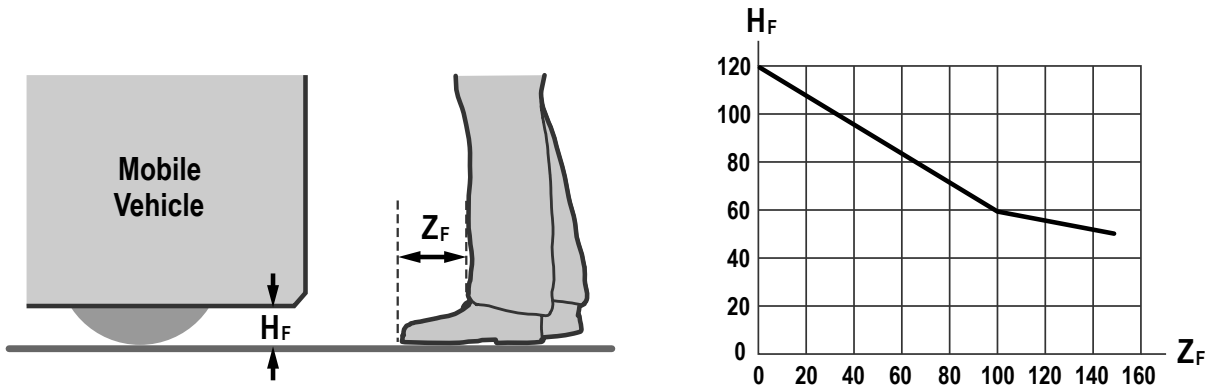
Figure 29. Diagram to determine the additional distance Z_F with lack of floor clearance H_F
