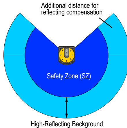
Figure 23. Reduce or remove a highly reflecting background
