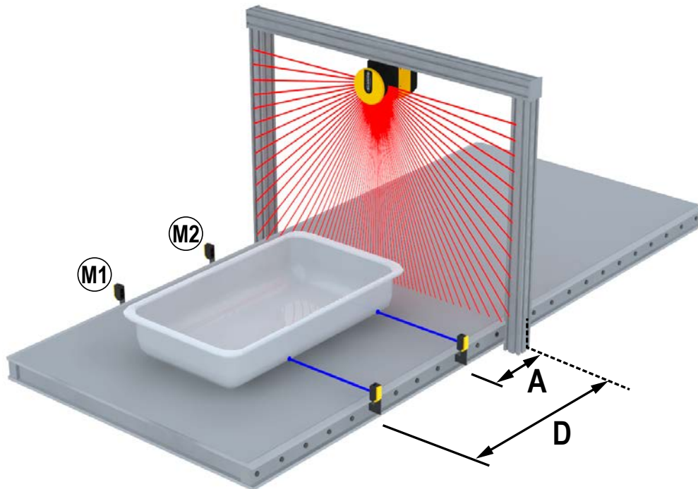
Figure 44. Muting function in the L configuration
