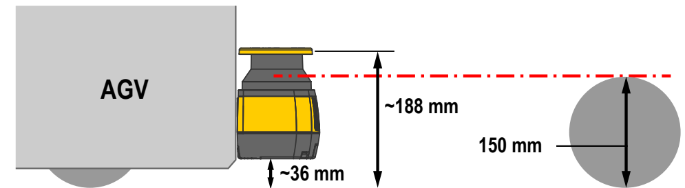
Figure 30. Diagram to determine the additional distance with lack of floor clearance
