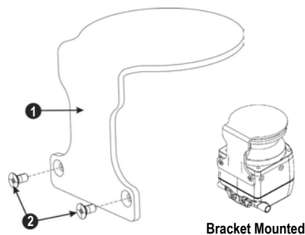
Figure 32. Mounting the protection bracket to the scanner
