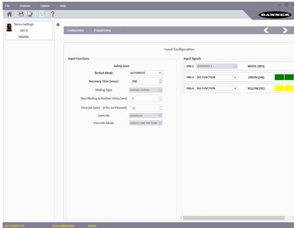
Figure 50. Input Configuration screen
