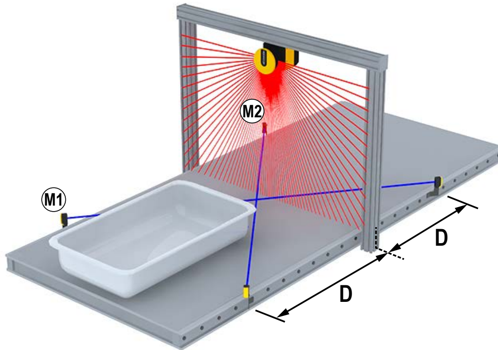
Figure 42. Muting function in the X configuration
