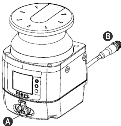
Figure 36. SX5 Safety Laser Scanner
