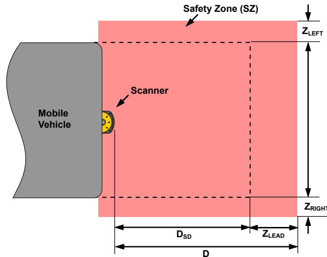
Figure 28. Calculating the minimum distance in a mobile vehicle application
