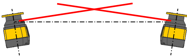
Figure 17. Scanners mounted at different scanning angles
