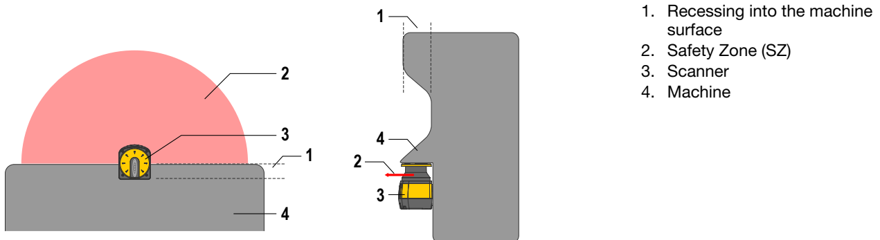
Figure 14. Mounting the scanner recessed into the machine
