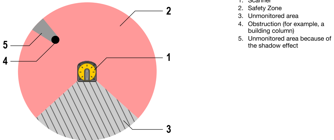
Figure 15. A shadow within the Safety Zone
