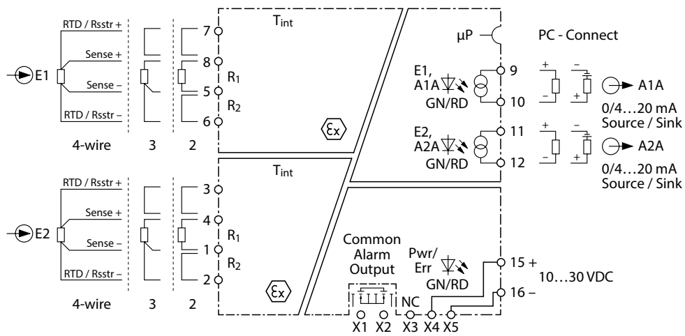
Abb. 6: IMX12-TI01-2RTDR-2
