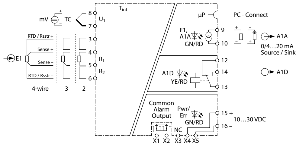
Abb. 11: IM12-TI02-1TCURTD-111R
