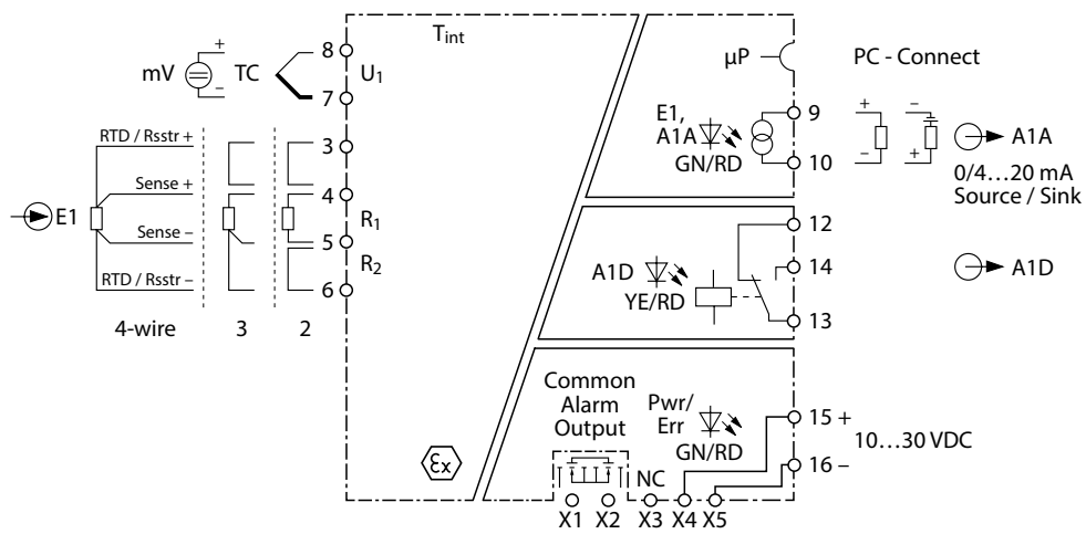
Abb. 10: IMX12-TI02-1CURTDR-111R
