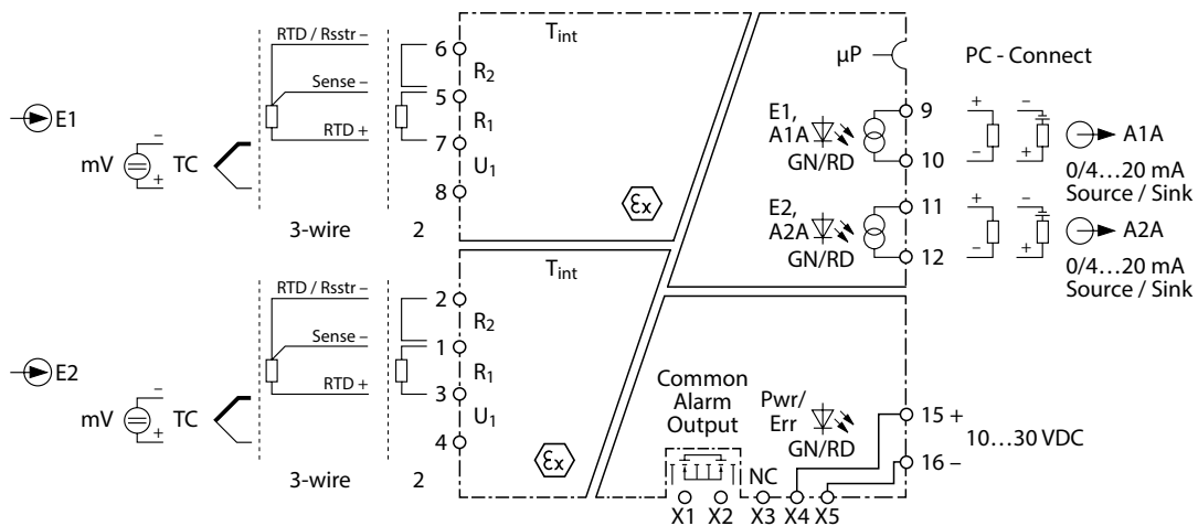
Abb. 8: IMX12-TI02-2TCURTD-2I
